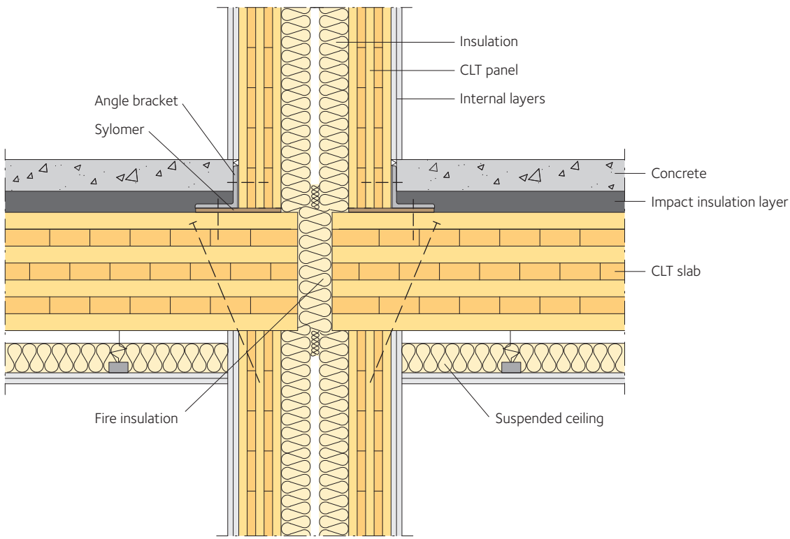
Figure 5.14 Internal party with acoustic separation floor-to-floor and wall-to-wall Note that the detail shown may not be suitable to meet fire regulations for buildings in multiple occupation in the UK.
