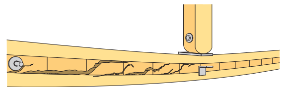
Figure 3.6 Rolling shear failure due to out-of-plane loading
