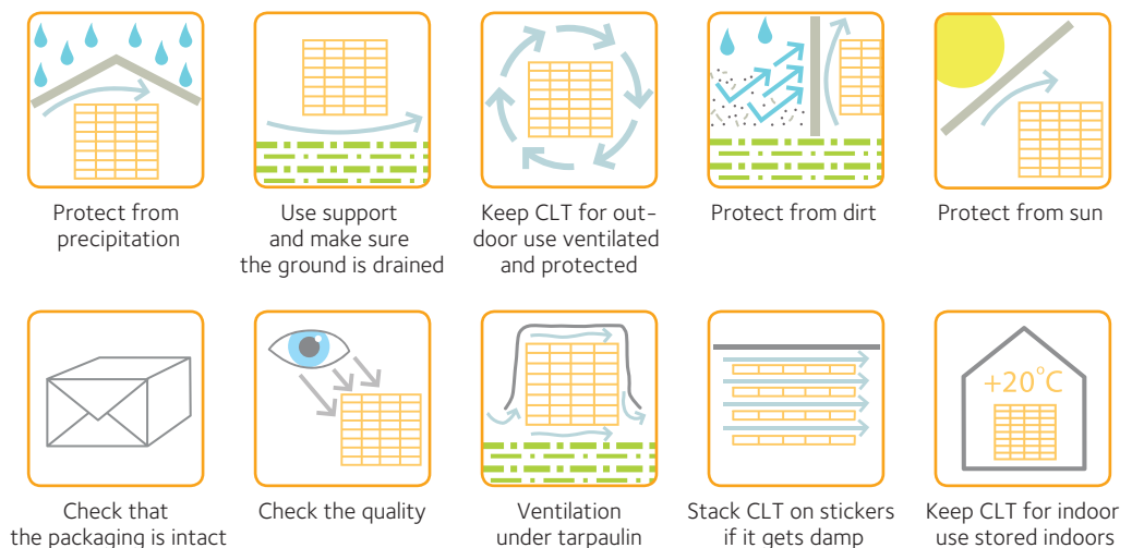
Figure 10.1 A few key principles for protecting CLT products
