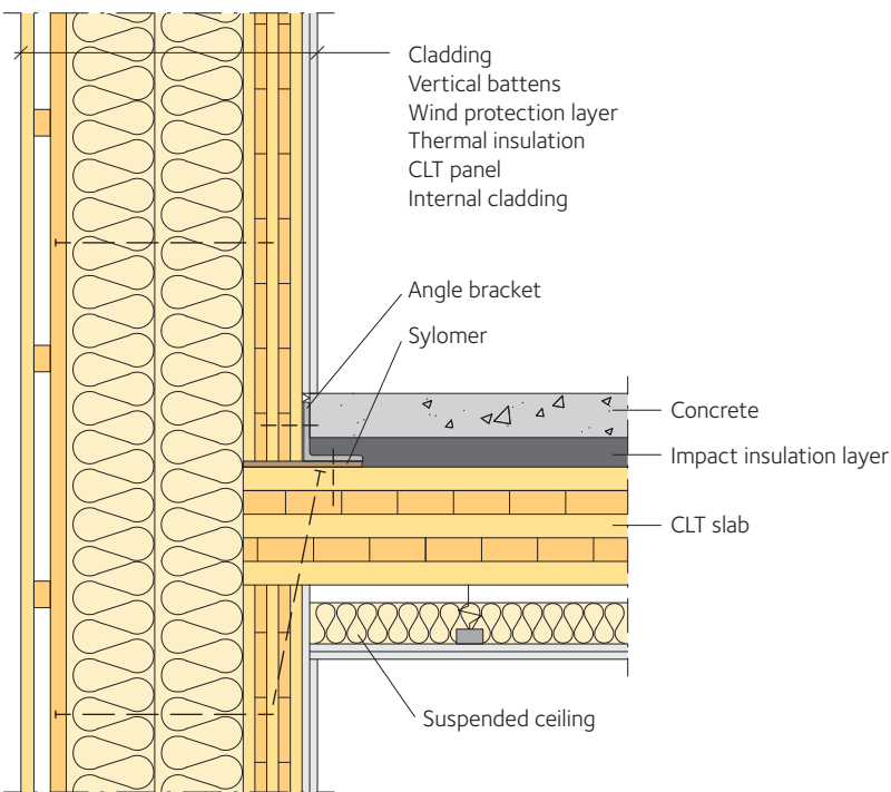
Figure 5.15 External wall with acoustic separation floor-to-floor Note that the detail shown may not be suitable to meet fire regulations for buildings in multiple occupation in the UK.
