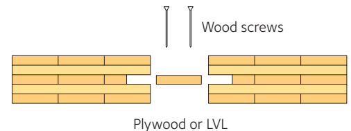
Figure 4.7 Joint with a loose tongue
